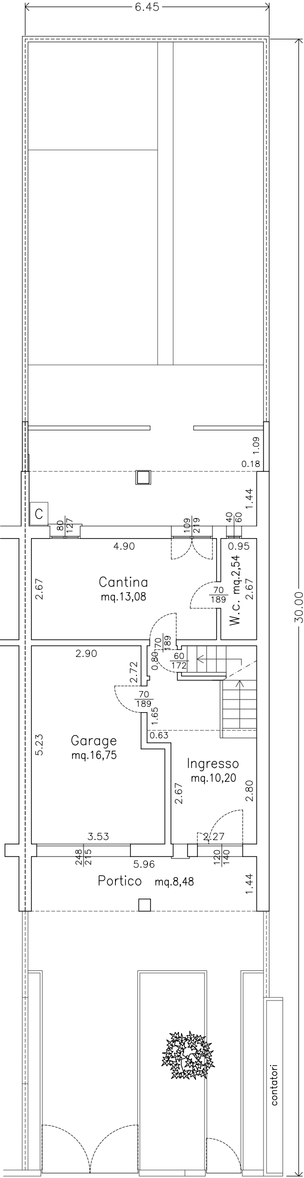
PIANO TERRA Scala 1:100
